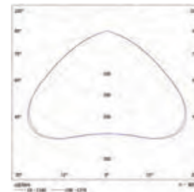
Symmetrical optics
